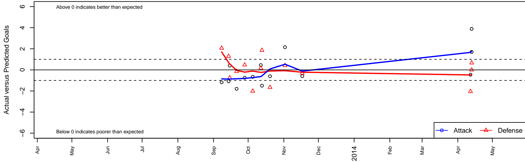
Sherman Oaks Extreme SC B97 Dots are actual minus expected GF (blue circles) and GA (red triangles). Blue line is smoothed change in attack strength. Red is smoothed change in defense strength.
